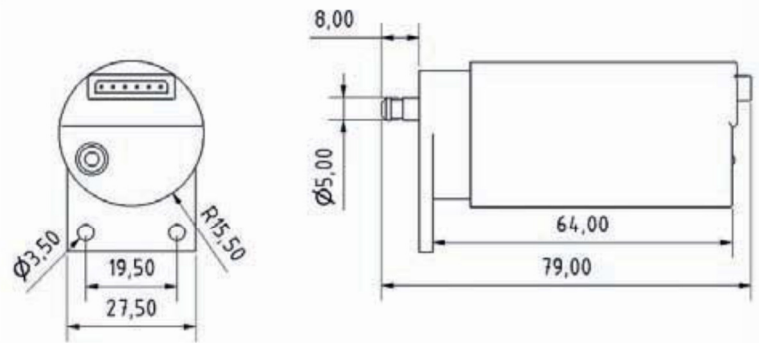
PowerBox™ Smoke Pump Dimensions
